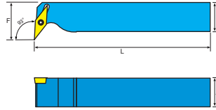
Tool holder
