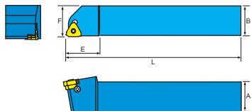
螺紋車刀架 Threading Tool Holder
