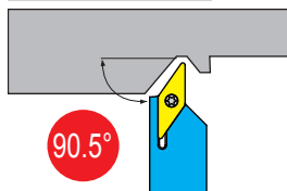
Tool holder
