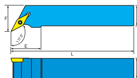
Tool holder
