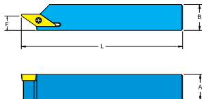
Tool holder
